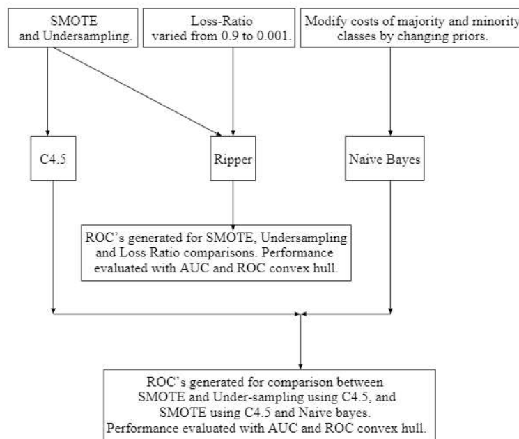
Figure 6: Experiments Overview
